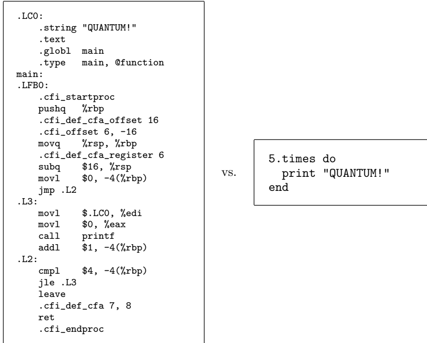
Figure 1.6 Contrasting a low-level and a high-level language for computer programs. The programs on the left and right perform the same task, but one is written in the low-level x86 assembly language, and one in the high-level language Ruby.
