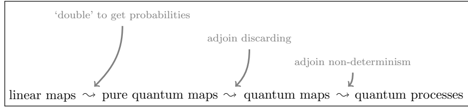
Figure 5.1 The passage from linear maps to quantum processes .
