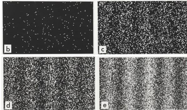
Figure 6.2 A more traditional double-slit experiment, involving a photographic plate. Note how interference fringes appear even when photons are sent one-by-one through a double slit. This exposes wave-like behaviour even for single photons.
