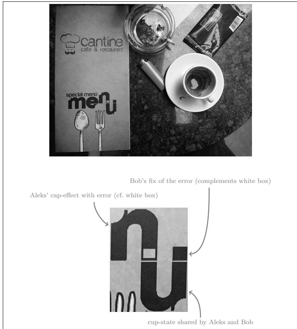
Figure 3.1 Teleportation is everywhere when you know how to recognise it. Here it is in the highly recommended Cafe Cantine in Istanbul's Taksim square area.
