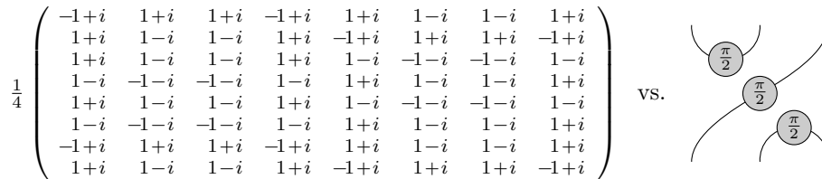
Figure 1.7 Contrasting a low-level and a high-level language for quantum processes, just like we contrasted the low-level and a high-level representation for digital data in Fig. 1.5, and a low-level and a high-level programming language in Fig. 1.6.
